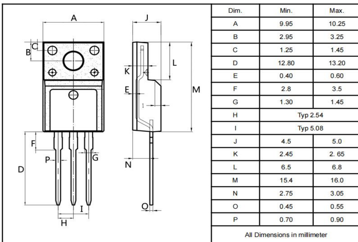
TO-220F
