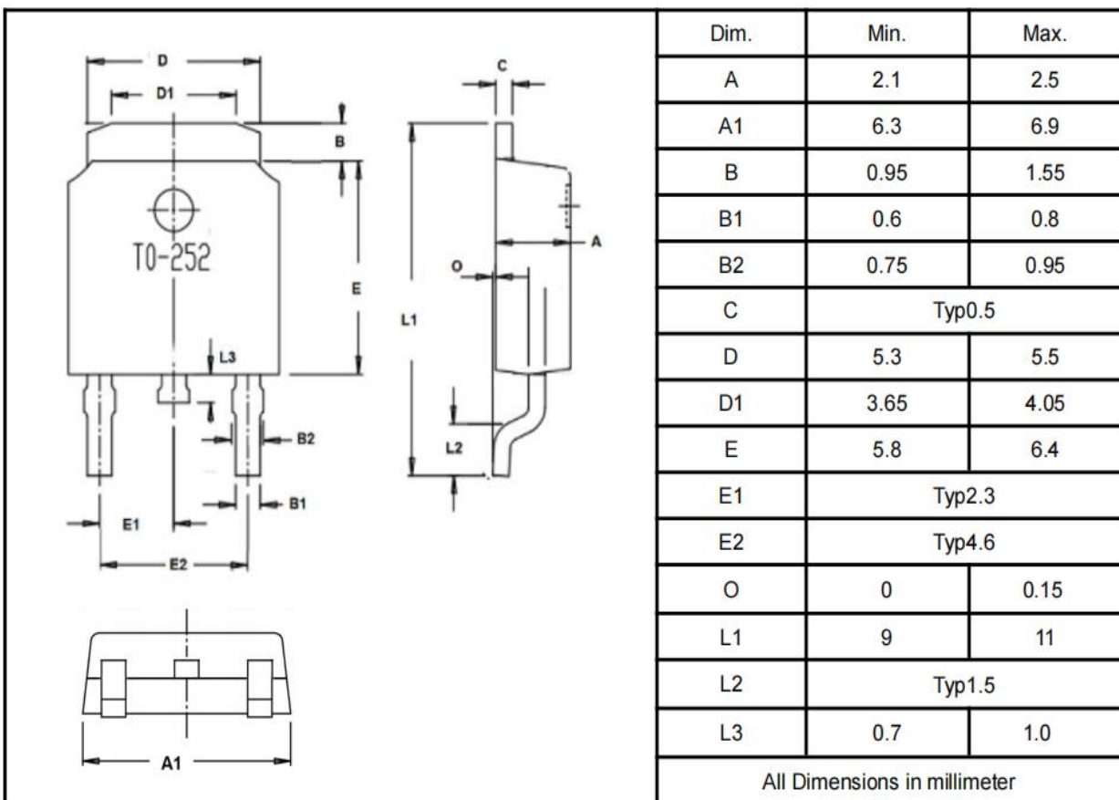
TO-252
